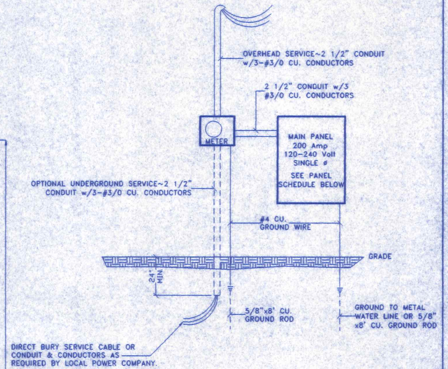
ELECTRICAL RISER DIAGRAM NO SCALE
