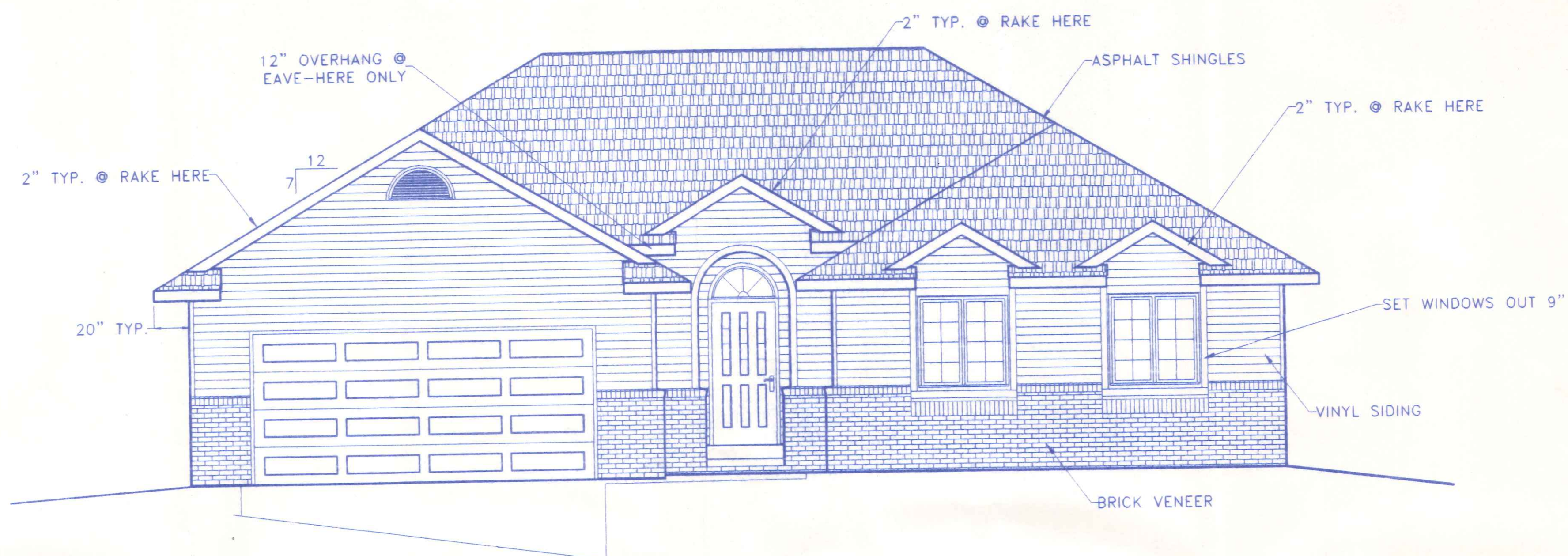
FRONT ELEVATION
