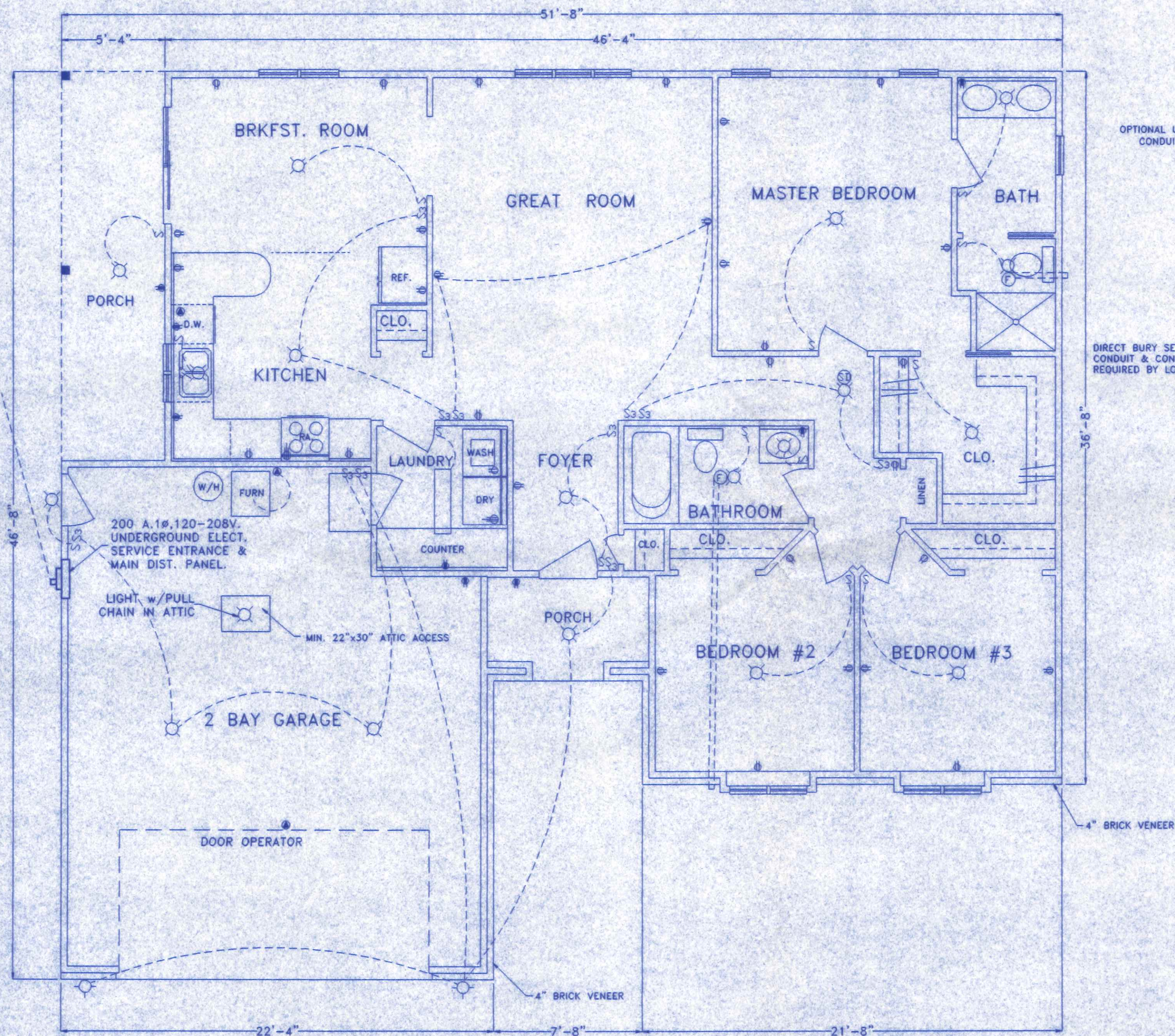
TYPICAL ELECTRICAL PLAN 1/4"=1'-0"
