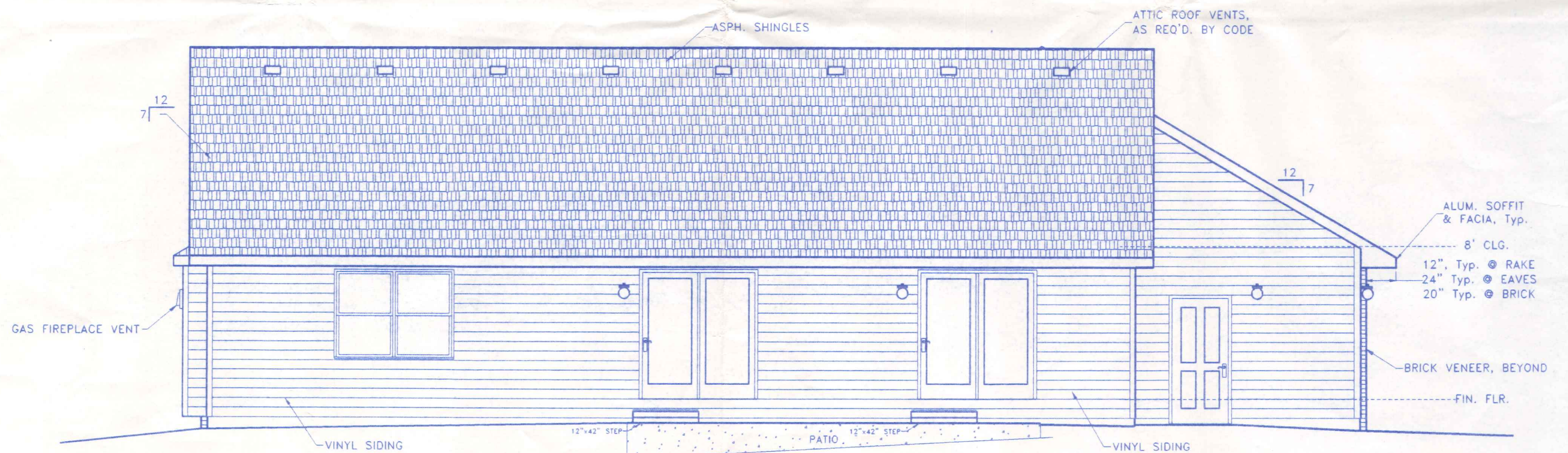
REAR ELEVATION
