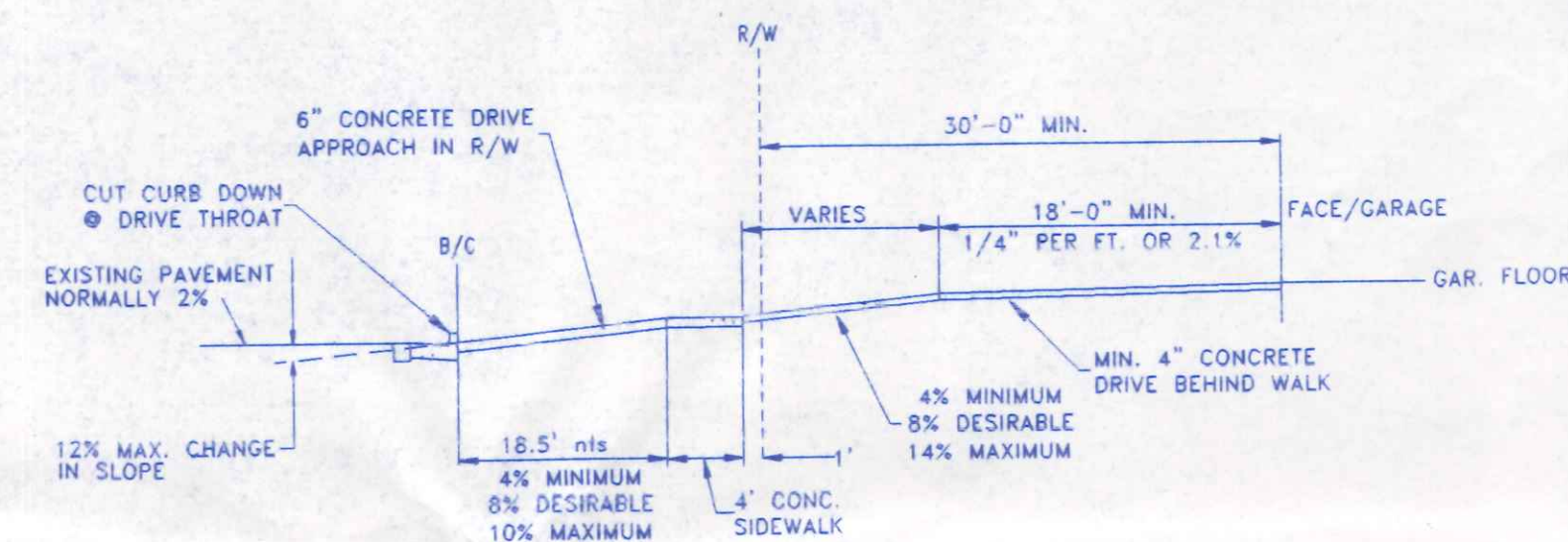
DRIVE APPROACH & GARAGE ELEVATION DETAIL
